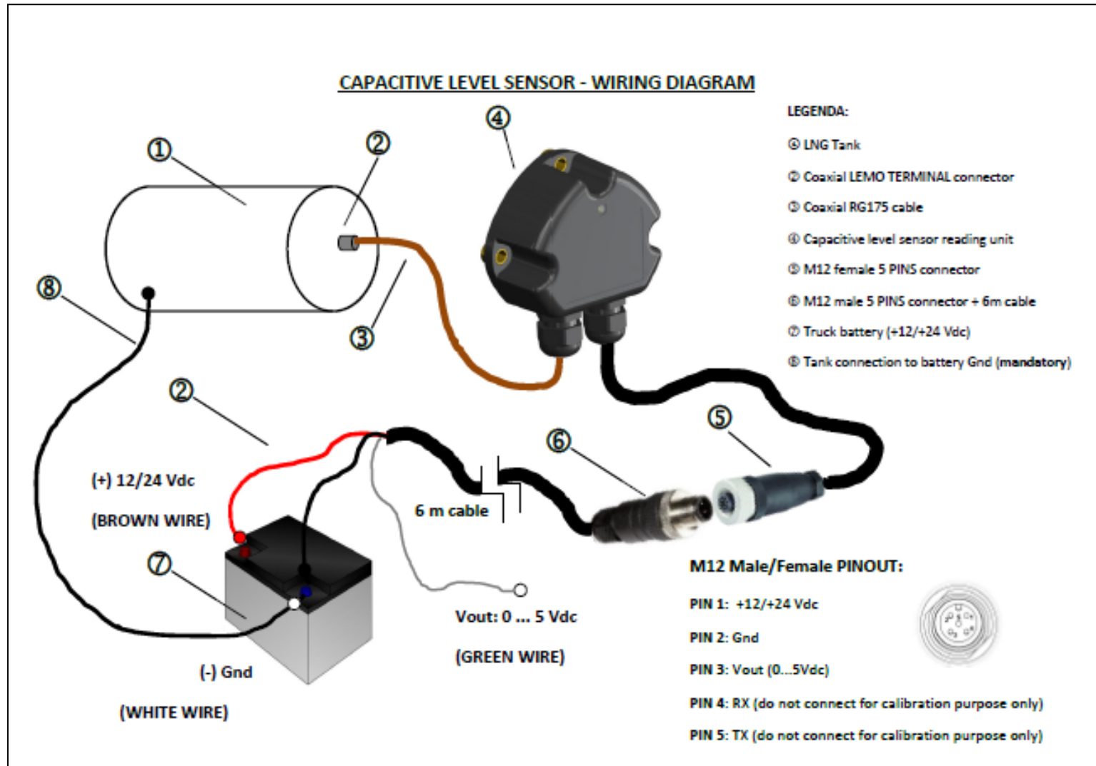
Figure 1 - Wiring Diagram.
